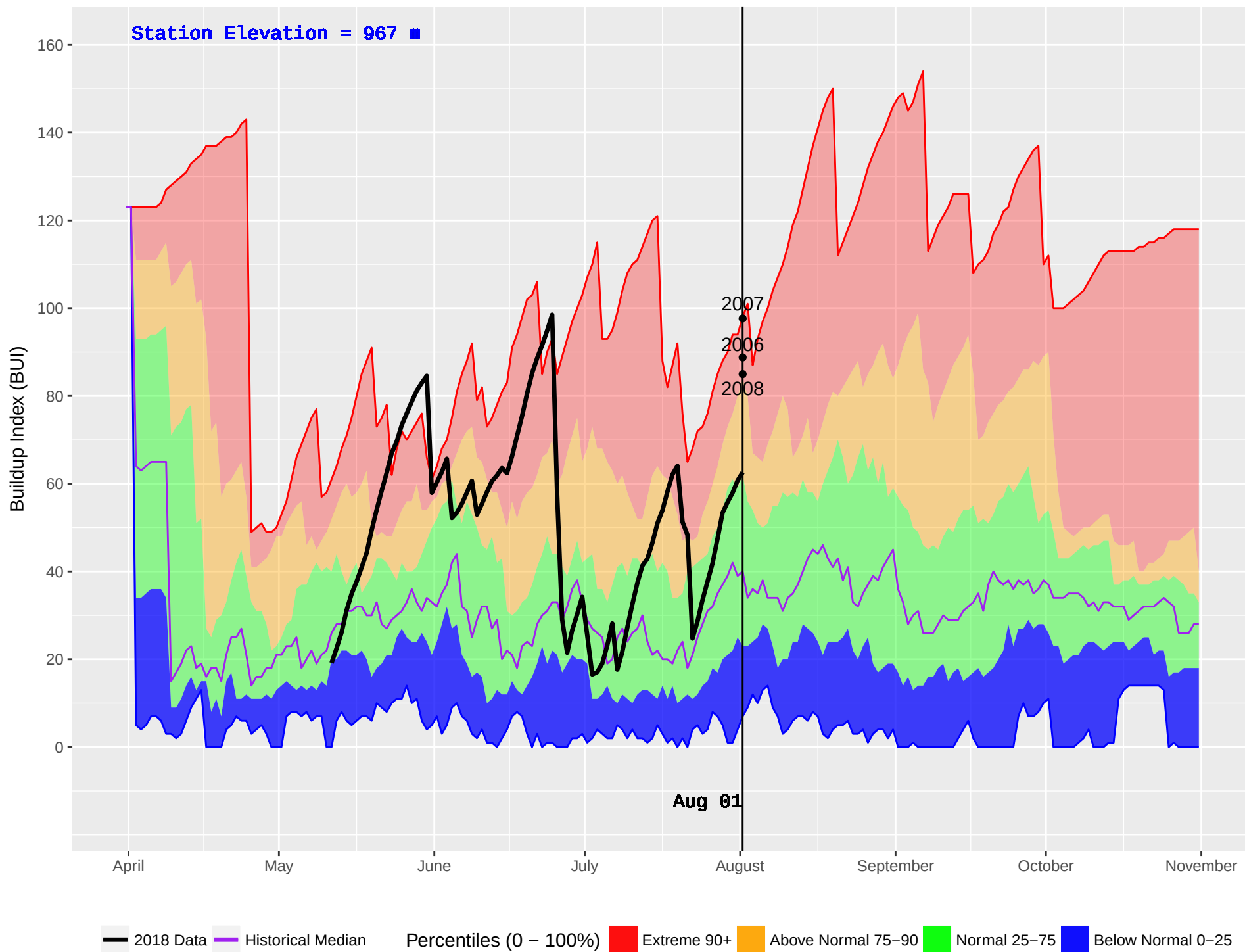
WONOWON (136) : Historical (1990–2016) and Current (2018) Daily Buildup Index (BUI)
