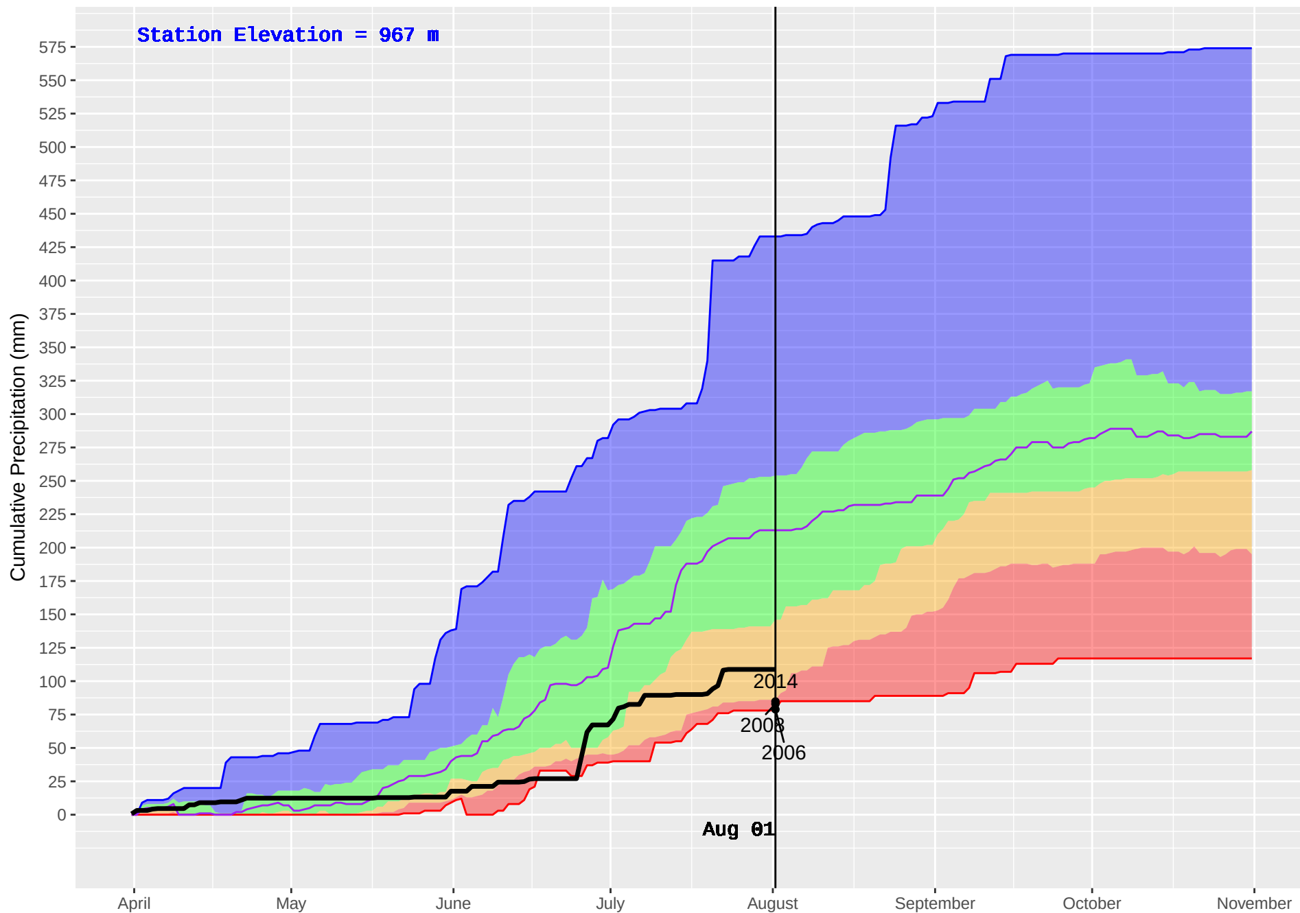
WONOWON (136) : Historical (1990–2016) and Current (2018) Daily Cumulative Precipitation
