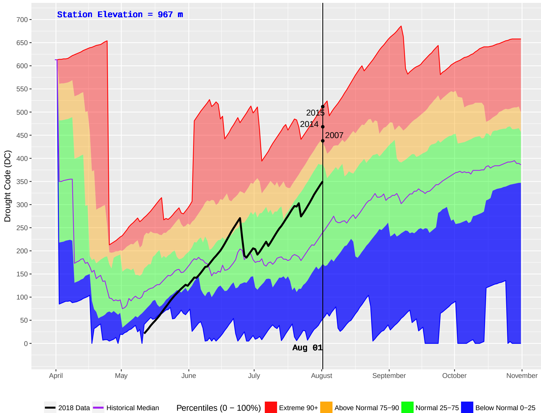
WONOWON (136) : Historical (1990–2016) and Current (2018) Daily Drought Code (DC)
