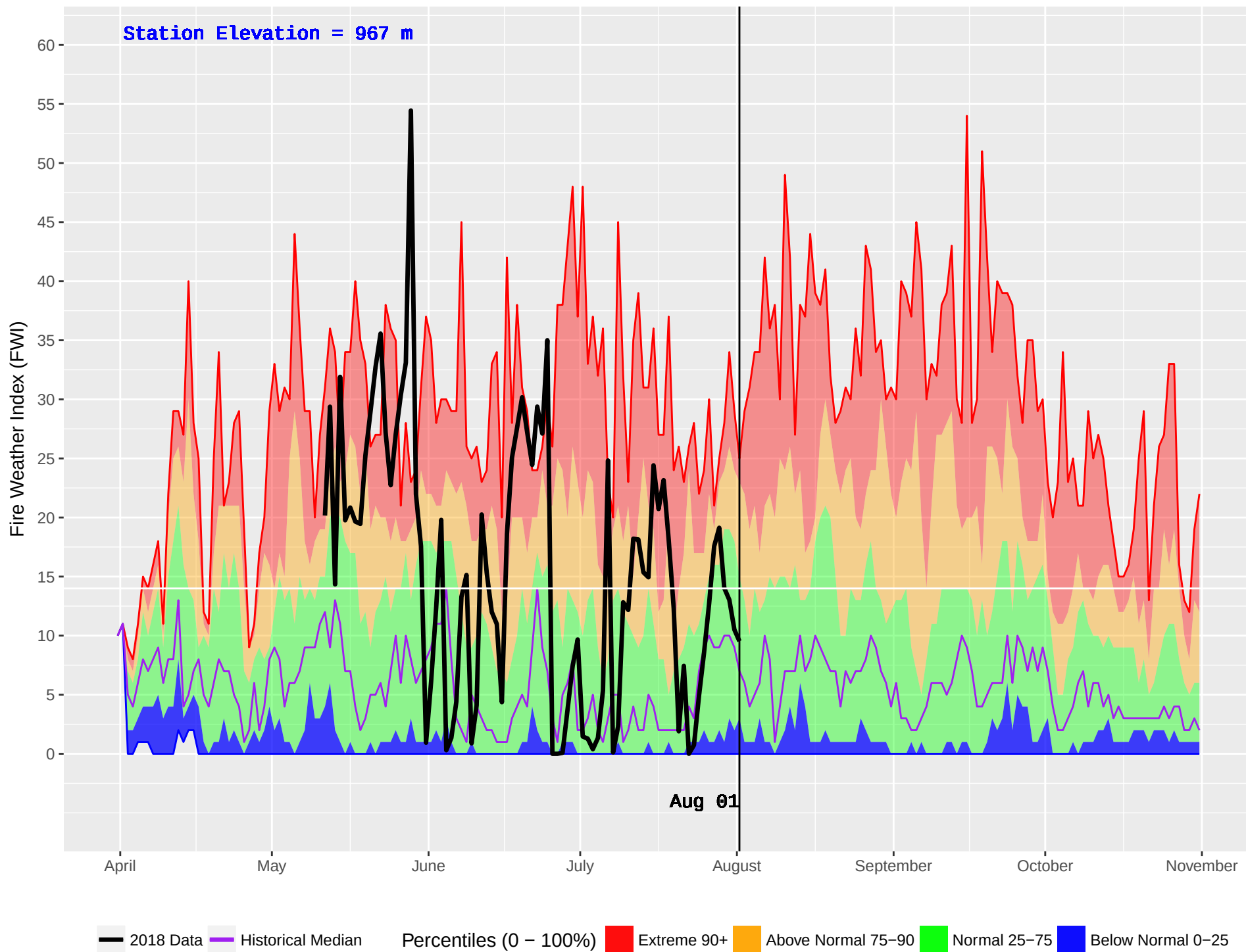
WONOWON (136) : Historical (1990–2016) and Current (2018) Daily Fire Weather Index (FWI)
