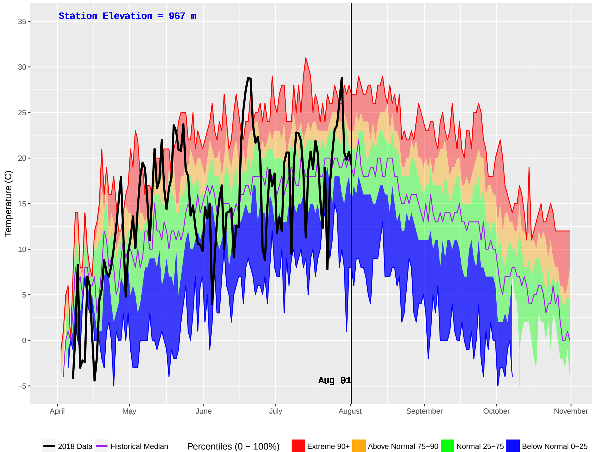
WONOWON (136) : Historical (1990–2016) and Current (2018) Daily Temperature
